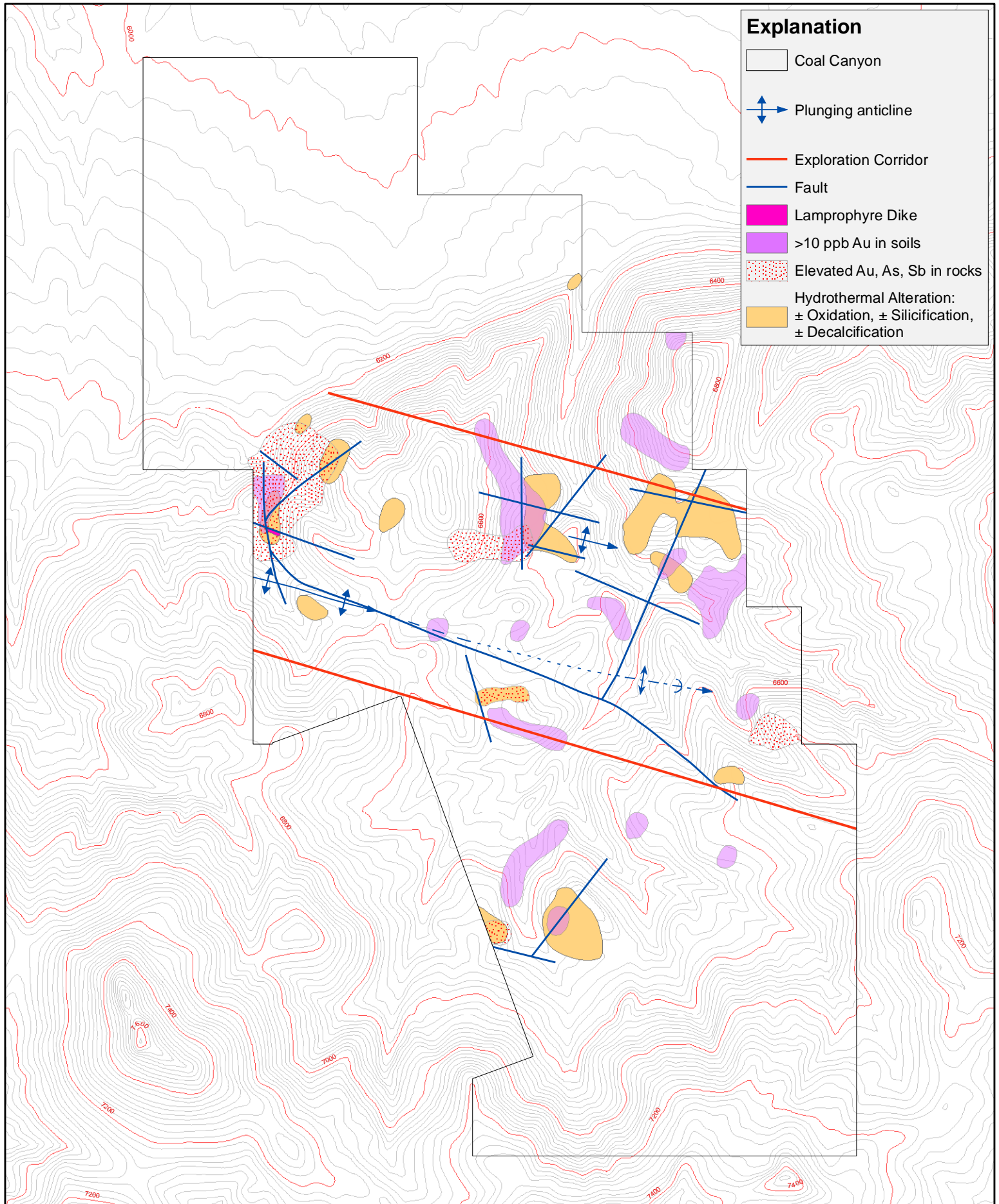
Fig. 3: WNW Fault / Fold Corridor
